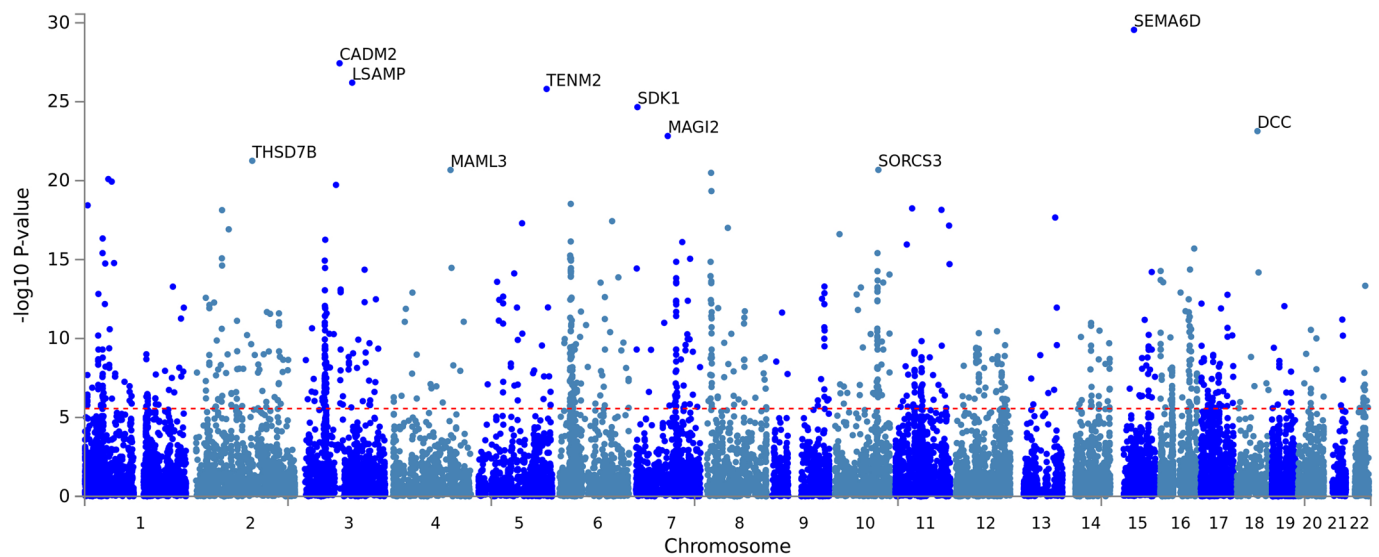
Extended Data Fig. 4 | MAGMA gene-based association analysis. Manhattan plot of the -\log_{10}(P) from a one-sided Z-test) of 18,093 genes that were tested for association in the MAGMA (v.1.08) gene-based association analysis (Supplementary Information section 6). The 10 most significant genes are labeled with gene names. Red dashed line represents Bonferroni-significance, adjusted for the number of tested genes (one-sided P = 2.74 \times 10^{-6} ). 928 genes were found to be significant, of which 244 have one or more genome-wide significant SNPs from the externalizing GWAS within their gene breakpoints. The results are also report in Supplementary Table 13.
